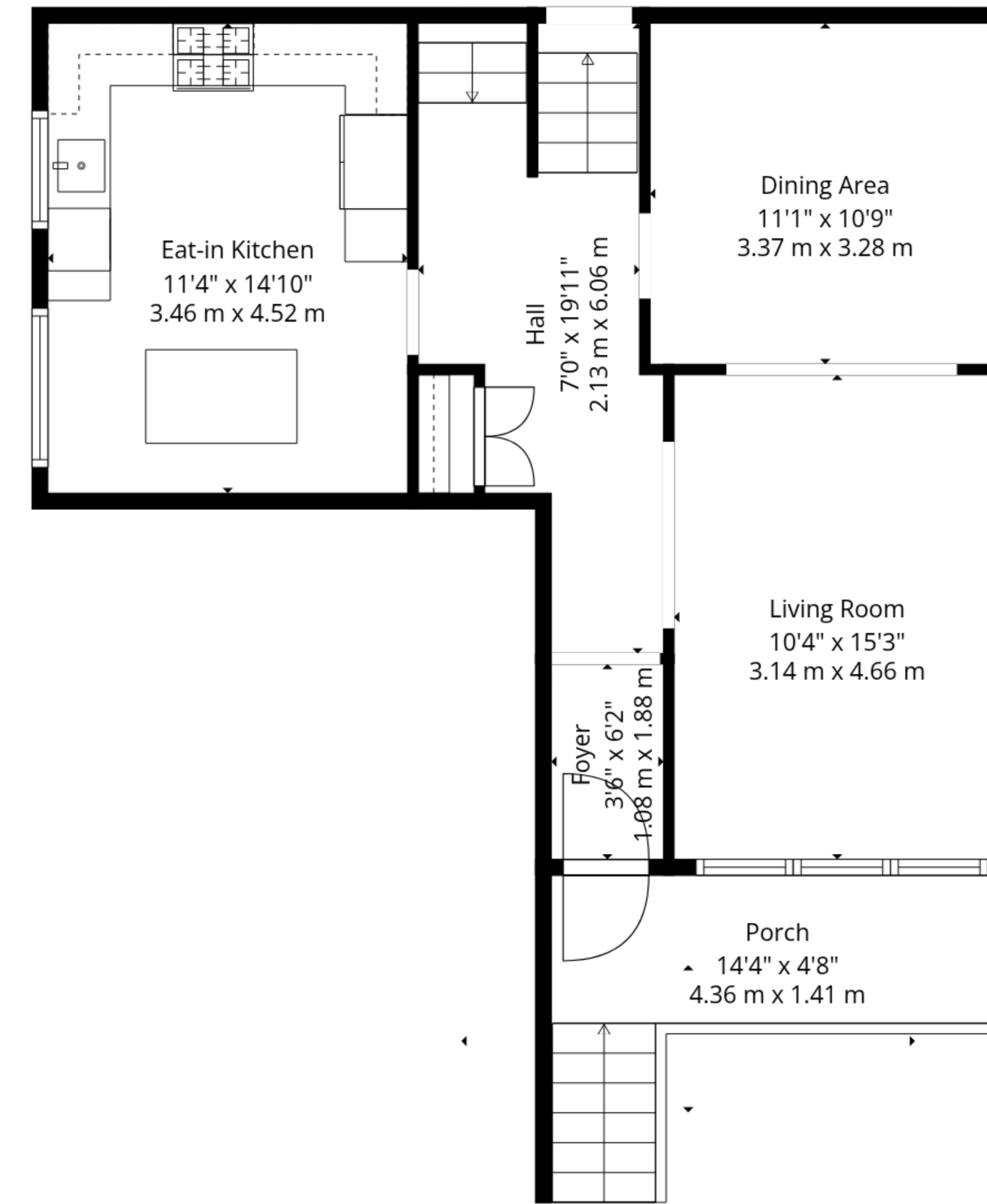
2nd Floor
